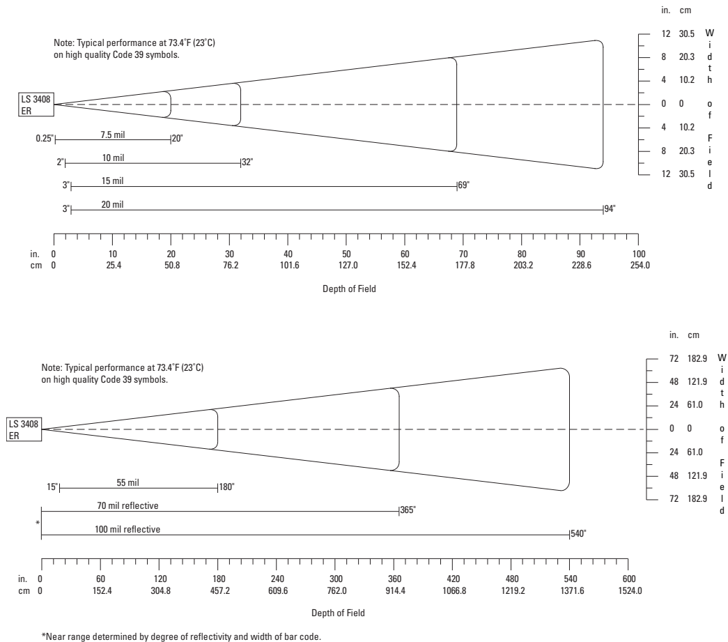
Figure 2-6 LS3408-ER Decode Zone
