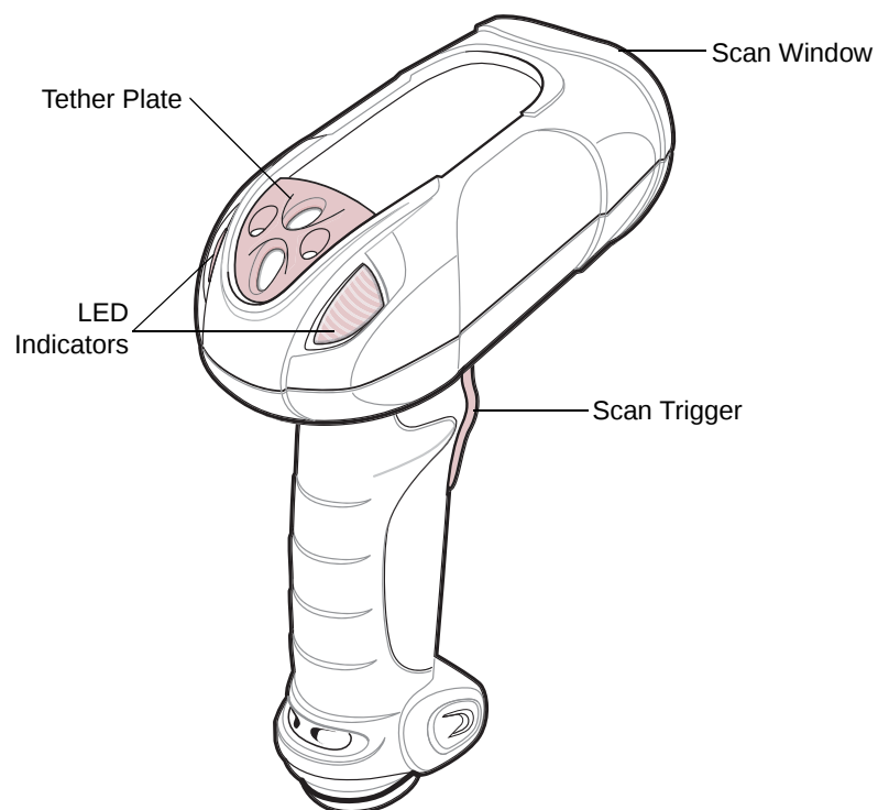
Figure 2-1 Parts
