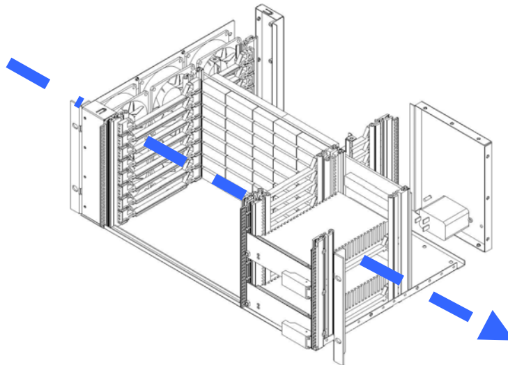
Figure 3-18 Air Flow
