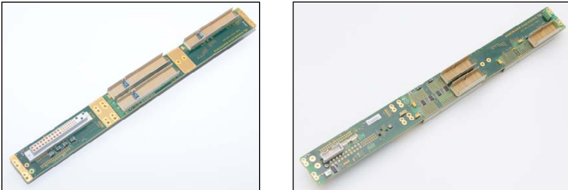
Figure 3-12 Backplane CPCI 9U 3 slot (6U) + PSU 47p (3U) front / rear
