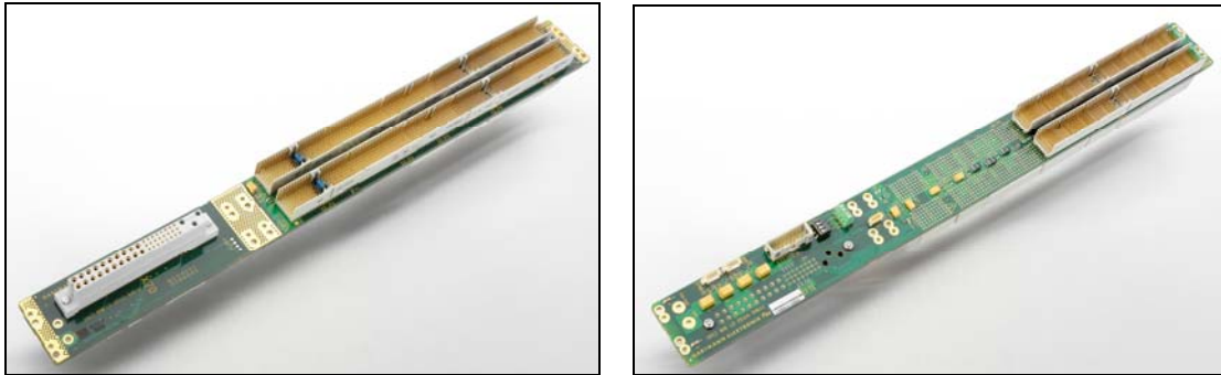
Figure 3-11 Backplane CPCI 9U 2 slot (6U) + PSU 47p (3U) front / rear
