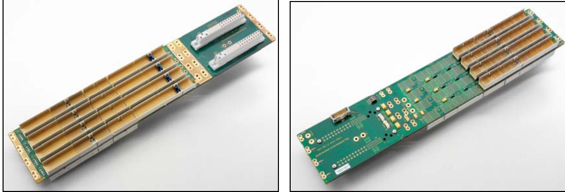
Figure 3-13 Backplane CPCI 9U 4 slot (6U) + 2 x PSU 47p (3U) front / rear
