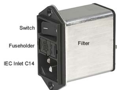
Figure 3-15 Power Entry Module
