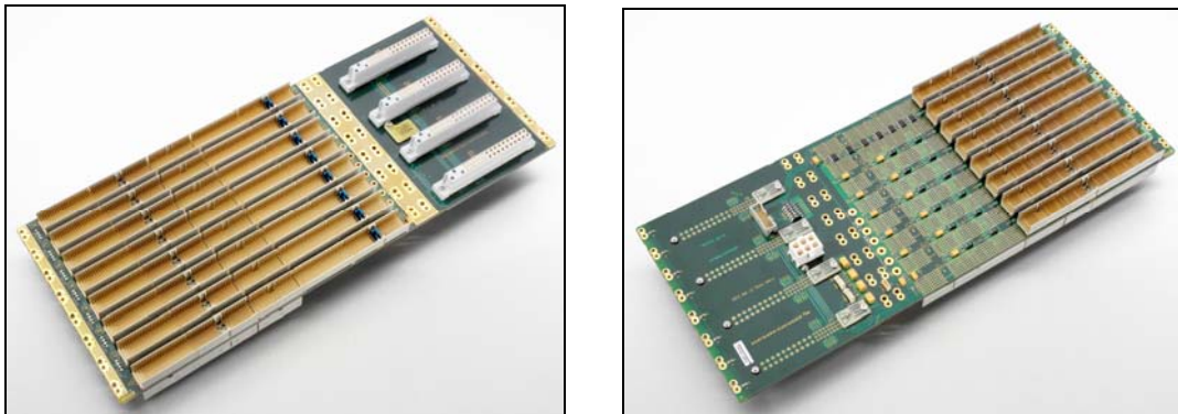
Figure 3-14 Backplane CPCI 9U 8 slot (6U) + 4 x PSU 47p (3U) front / rear
