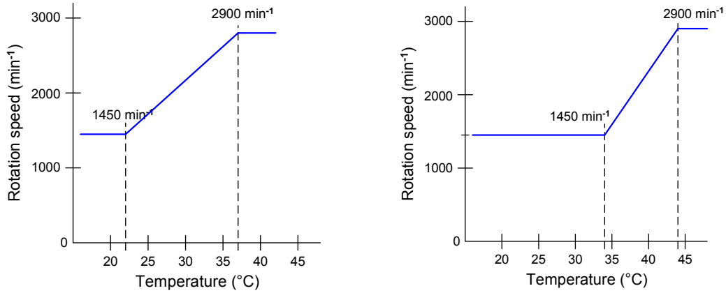
Figure 3-9 Fan characteristic dip-switch on/off
