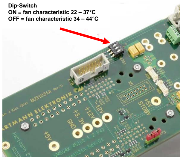
Figure 3-8 Dip-Switch
