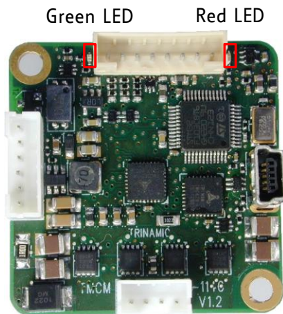
Figure 6.1 On-board LEDs
