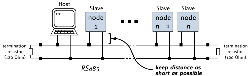
Figure 4.3 Bus structure
