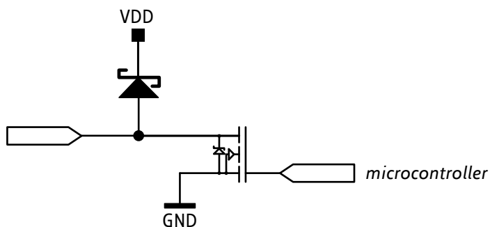
Figure 4.8 General purpose output OUT_0
