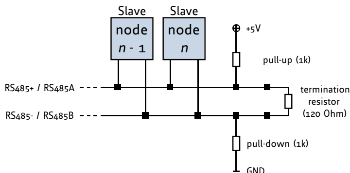
Figure 4.4 Bus lines with resistor network
