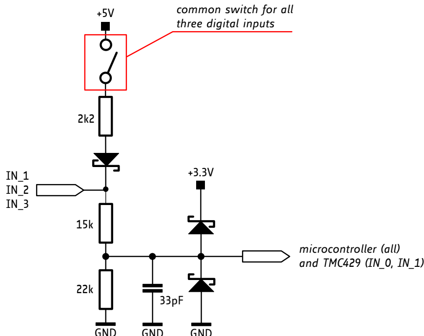
Figure 4.6 General purpose inputs (simplified input circuit)
