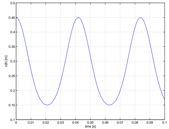
Figure 3.6. Case 1: Horizontal position of the sliding block.
