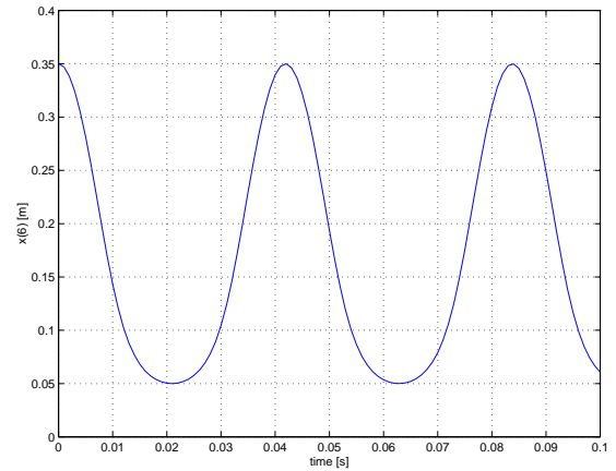
Figure 3.12. Case 2: Horizontal position of the sliding block.
