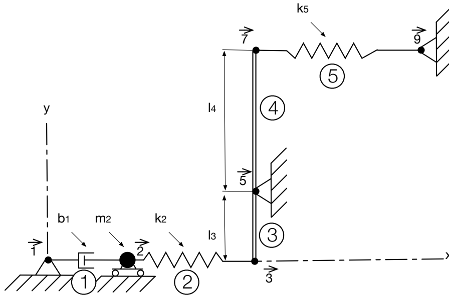
Figure 3.38. Lever system.
