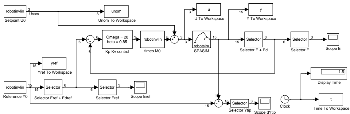
Figure 3.50. Block diagram for a closed-loop simulation of the motion of the manipulator mechanism using SIMULINK. Most signals are vectors and the numbers indicate the size of the vectors.
