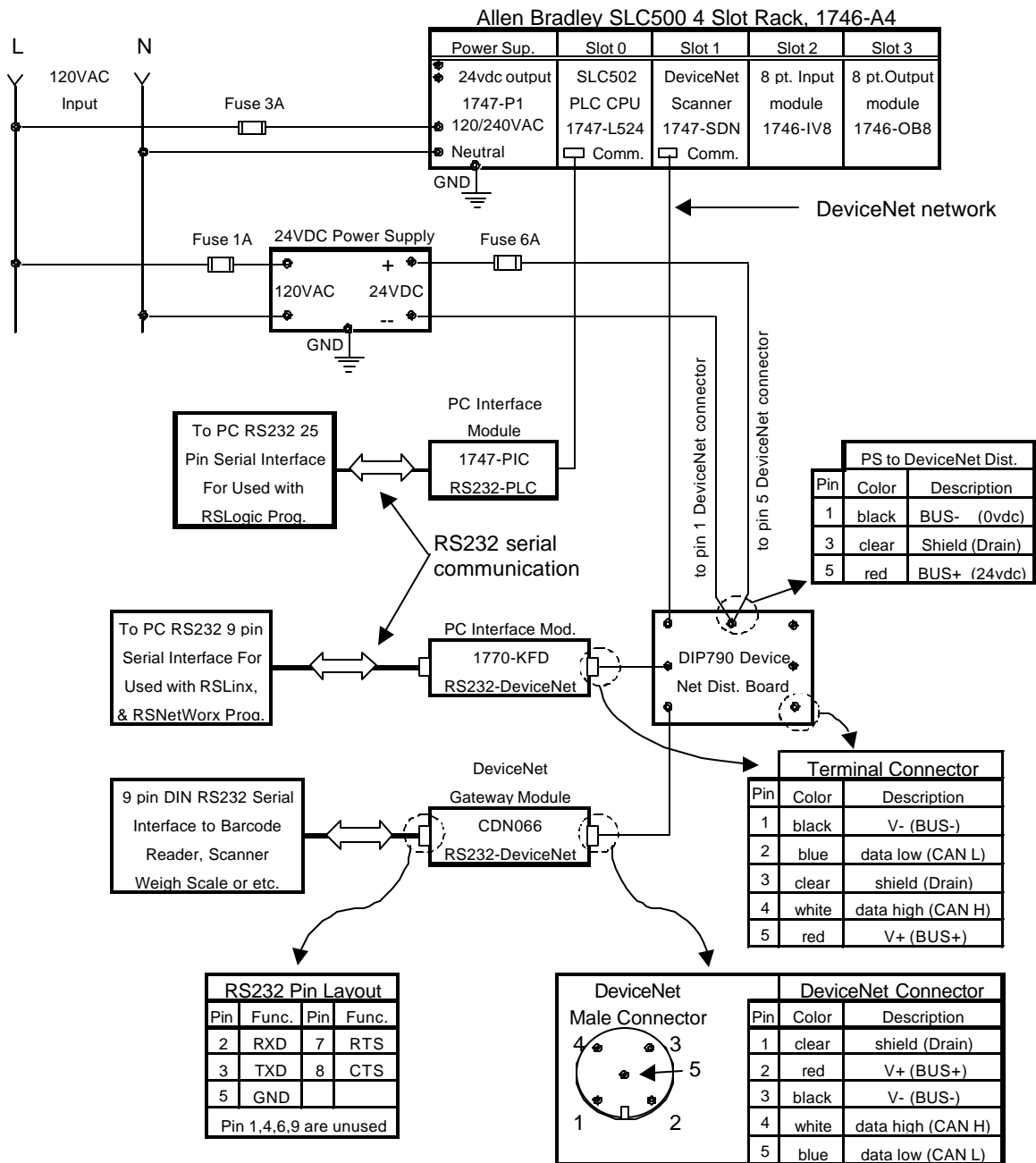
Figure 1. CDN066 Integrated with Allen Bradley SLC500
