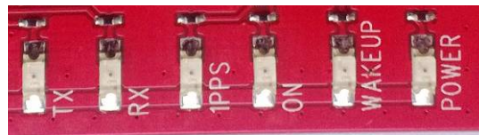
Figure 7: EVA2135-H LED's
