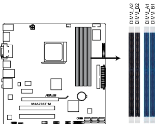
M4A785T-M 240-pin DDR3 DIMM sockets
