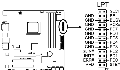
M4A785T-M Parallel Port Connector
