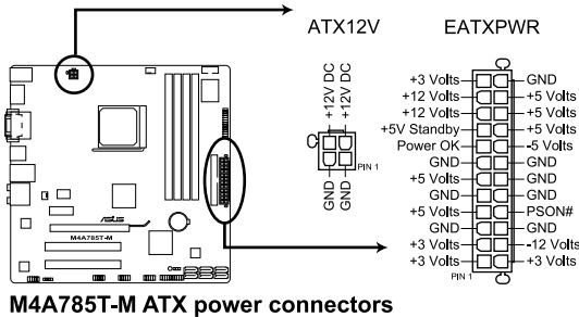
M4A785T-M ATX power connectors
