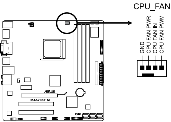
M4A785T-M CPU fan connector
