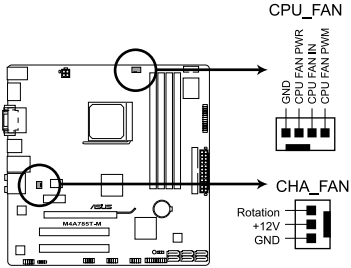
M4A785T-M fan connectors
