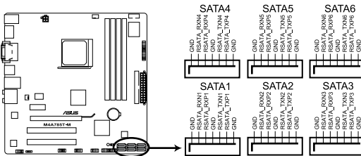
M4A785T-M SATA connectors
