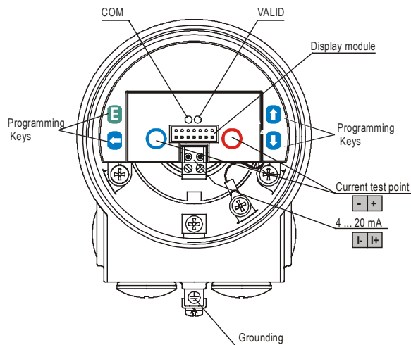
Transmitter with removed cover
