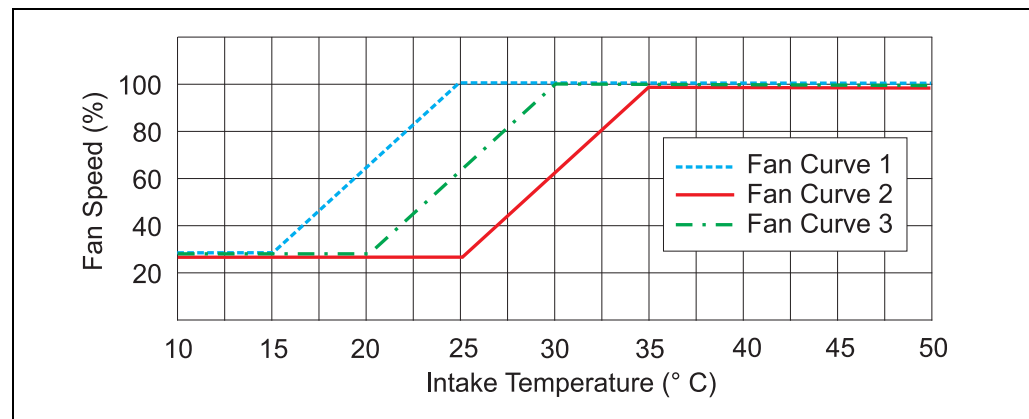
Figure 11: Fan curves, temperature measured at intake NTC
