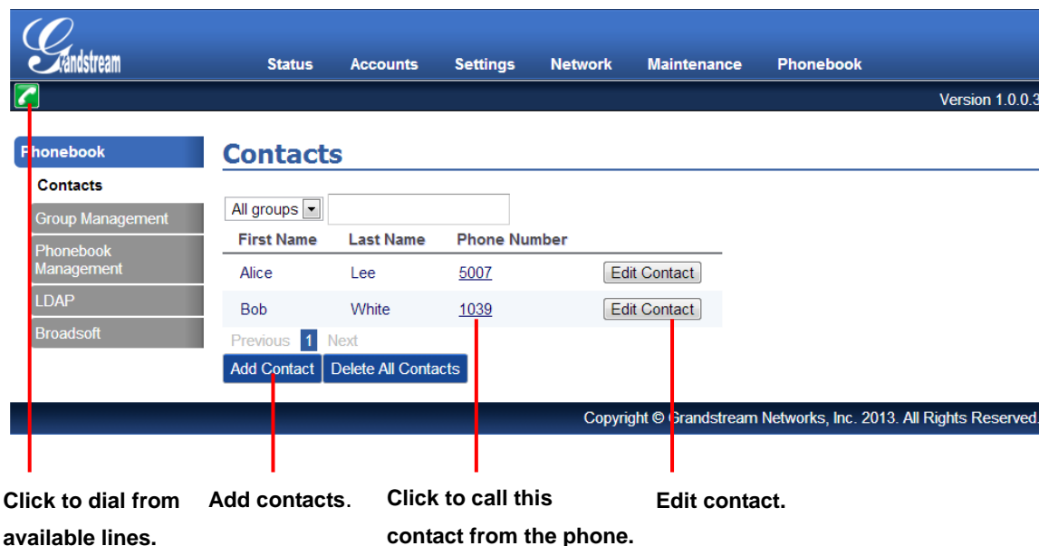
Figure 3: Web GUI - Phonebook->Contacts
