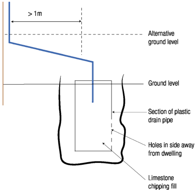
Figure 6 Suggestion for condensate soakaway drain
