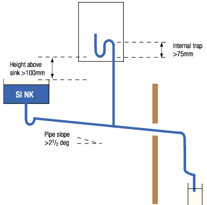
Figure 5 Connection to internal sink waste (downstream of sink trap)
