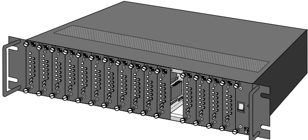
Figure 4. Model 1000R16P Rack Chassis with Power Supply
