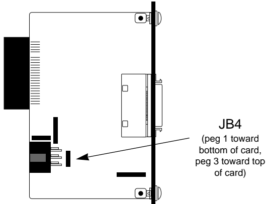
Figure 2. Rear card jumper location
