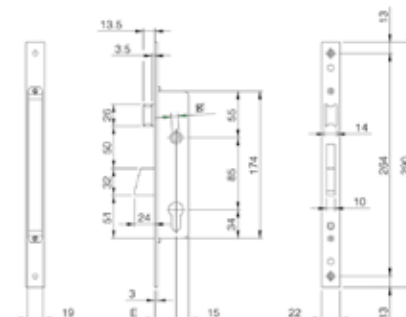
Reversible Latch
