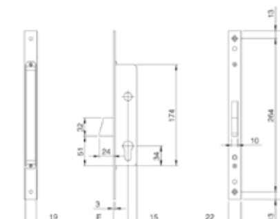
Bolt Throws 24mm
