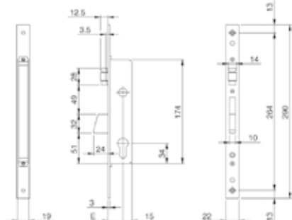
Adjustable Roller
