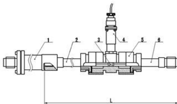
LWGY 4~10 Sensor Structure & Installation Diagram
