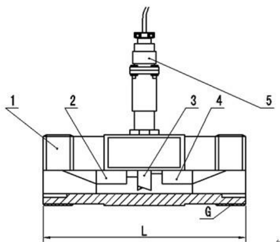
LWGY 15~40 Sensor Structure & Installation Diagram
