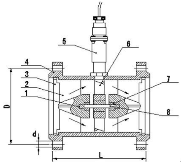
LWGY 50~200 Sensor Structure &amp; Installation Diagram
