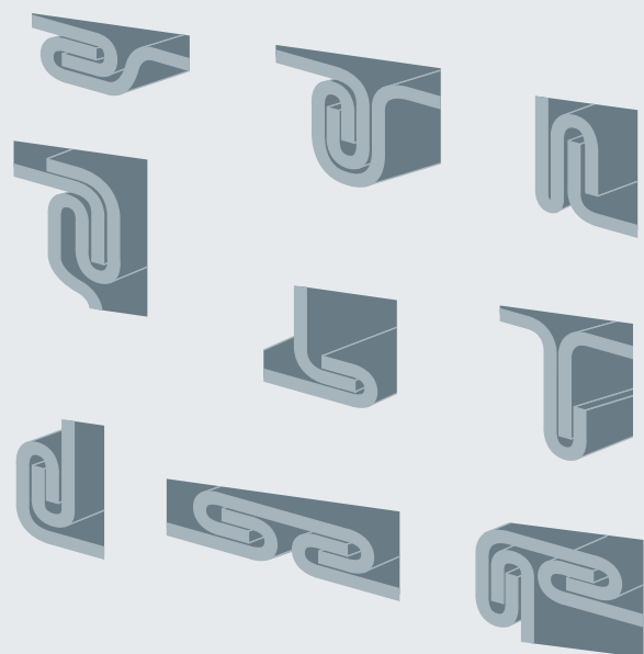
Different single and double lock seams
