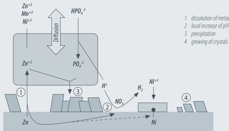
Phosphating
