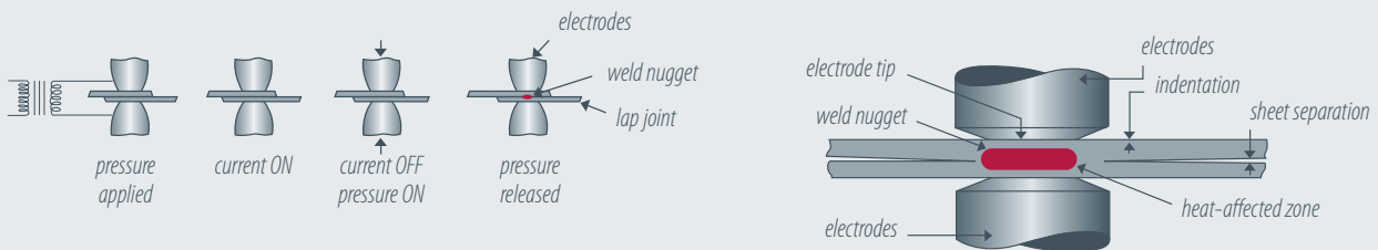
Spot welding
