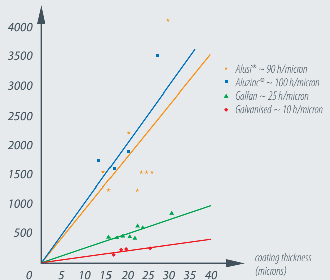
Resistance to salt spray on flat samples
