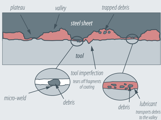
Galling
