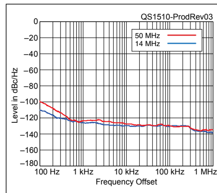
Figure 3 — Spectral display of the ANAN-100D transmitter output during phase noise testing. Power output is 100 W on the 14 MHz band (blue trace) and on the 50 MHz band (red trace). The carrier, off the left edge of the plot, is not shown. This plot shows composite transmitted noise 100 Hz to 1 MHz from the carrier. The reference level is 0 dBc, and the vertical scale is in dBc/Hz.
