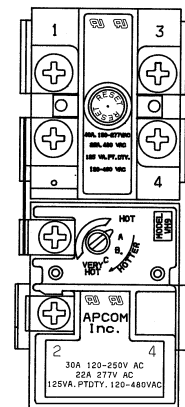
LOWER THERMOSTAT ADJUSTABLE BEHIND LOWER ACCESS PANEL
