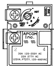
LOWER THERMOSTAT ADJUSTABLE BEHIND LOWER ACCESS PANEL
