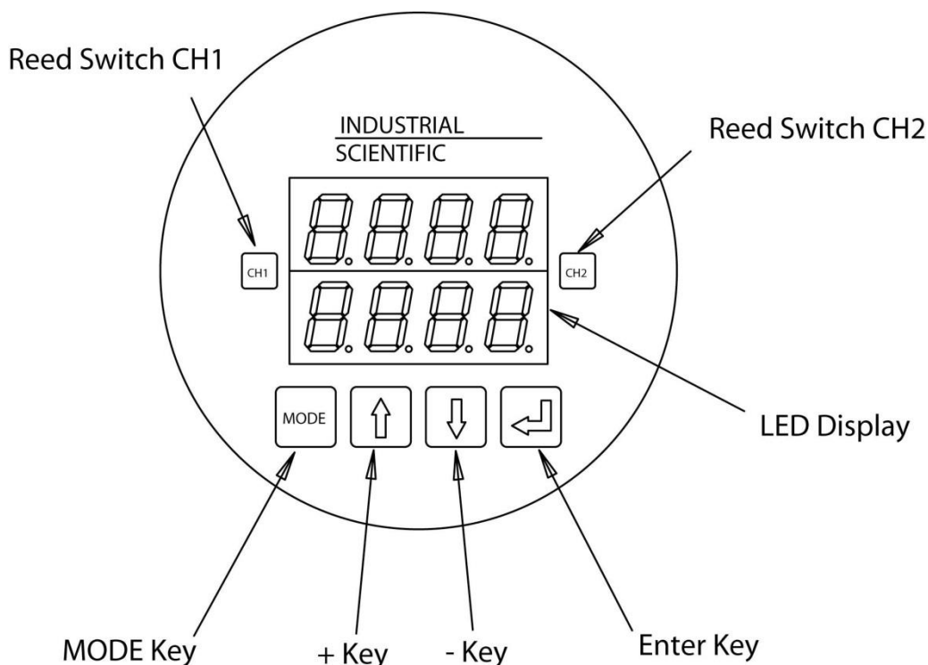
Figure 2-3. Locations of iTrans ™ERREUR ! SOURCE DU RENVOI INTROUVABLE. Input Keys and Reed Switches
