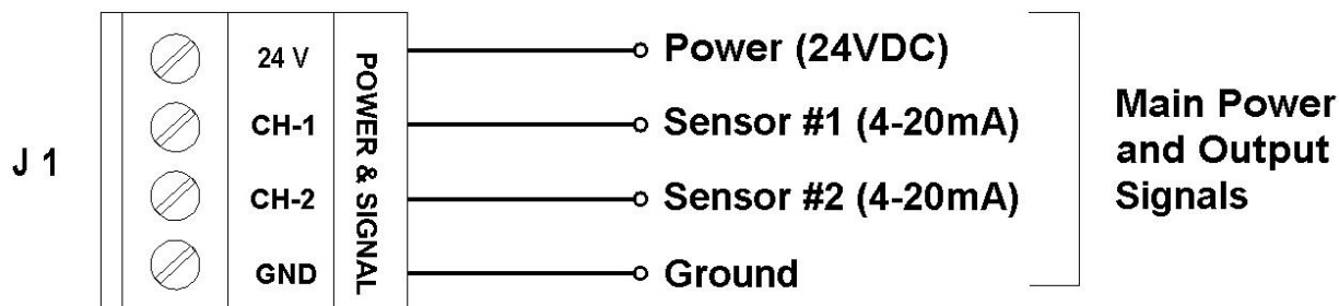
Figure 4-2. Power and Signal Connector J1 on the iTrans ERREUR ! SOURCE DU RENVOI INTROUVABLE .
