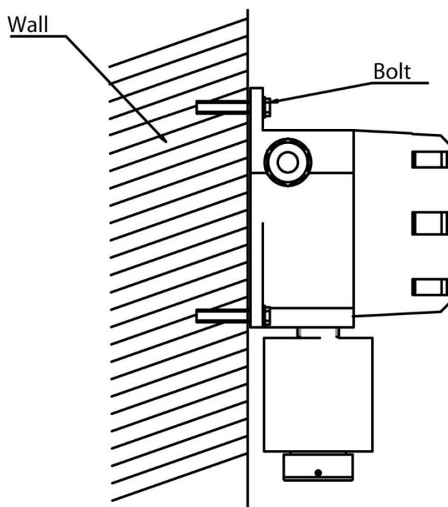
Figure 3-1. Mounting the iTrans ERREUR ! SOURCE DU RENVOI INTROUVABLE. Gas Monitor on a Wall
