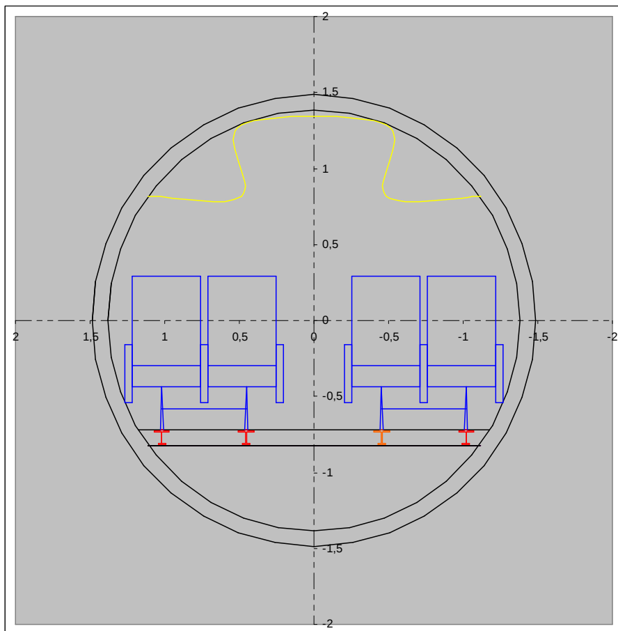
Figure 3.4 Fuselage Cross Section Sketch
