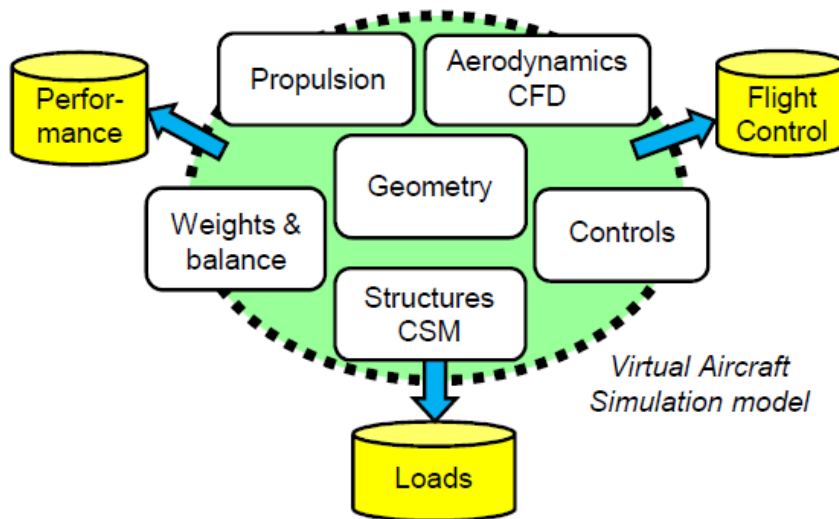
Figure 2.5 CEASIOM Virtual Aircraft Simulation Model (CEASIOM 2010)
