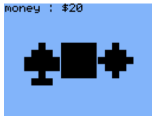
Figure 11.10.: Jackpot
