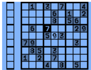
Figure 11.25.: Sudoku
