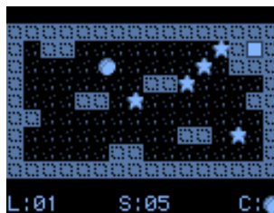
Figure 11.24.: Star game
