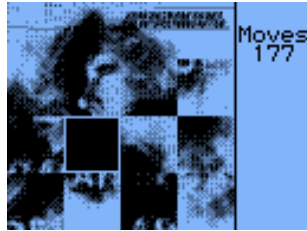
Figure 11.18.: Sliding puzzle
