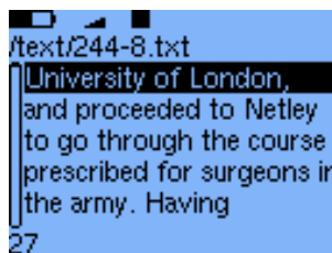
Figure 11.42.: A bookmark
