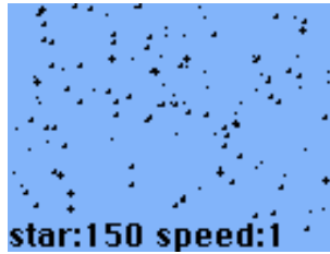
Figure 11.38.: Starfield
