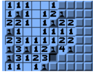
Figure 11.13.: Minesweeper plugin
