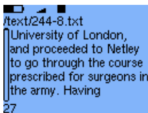
Figure 11.40.: Text Viewer
