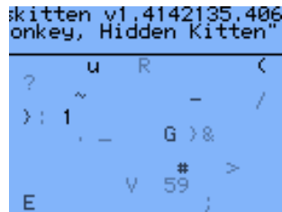
Figure 11.16.: Robotfindskitten
