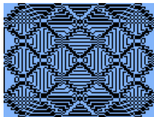
Figure 11.33.: Mosaïque
