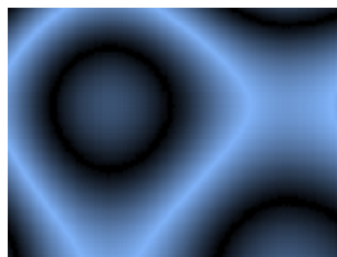
Figure 11.36.: Plasma
