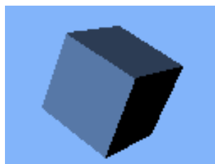
Figure 11.29.: Cube
