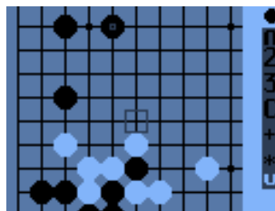
Figure 11.8.: Goban
