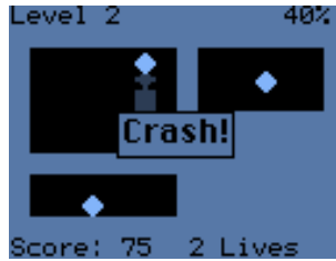
Figure 11.27.: Xbox
