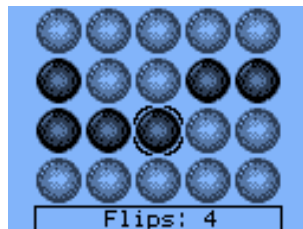
Figure 11.7.: Flipit
