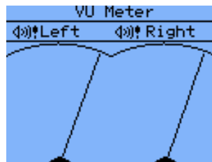
Figure 11.39.: VU-Meter
