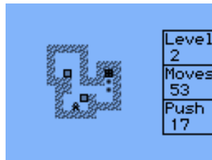
Figure 11.21.: Sokoban
