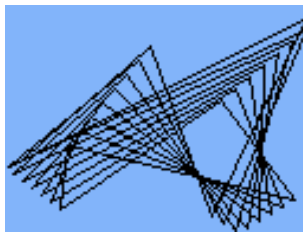
Figure 11.30.: Demystify
