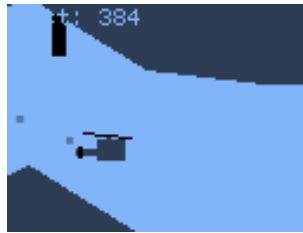
Figure 11.5.: Chopper
