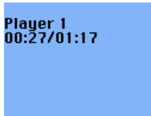
Figure 11.45.: Chess Clock
