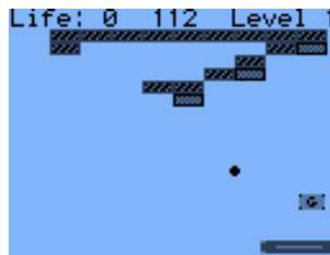
Figure 11.2.: BrickMania
