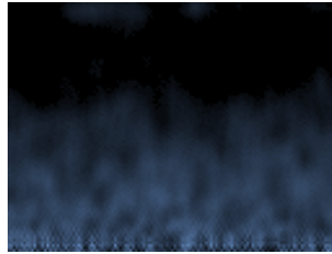
Figure 11.31.: Fire
