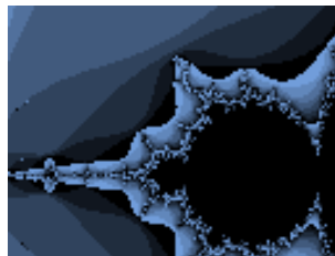
Figure 11.32.: Fractals: Mandelbrot set
