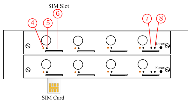
Figure 1-3-3 Back Panel
