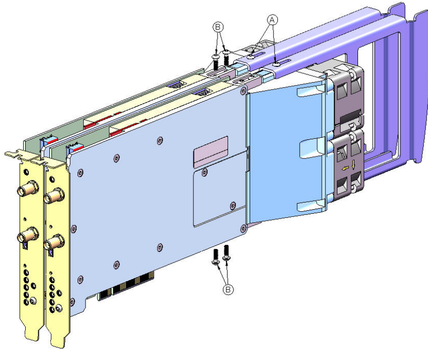
Diagram showing fan/support assembly fixings ( U5303A shown as example)
