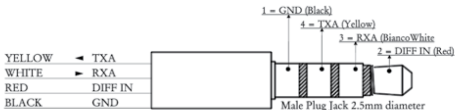
Fig. 15 - I/O Connector
