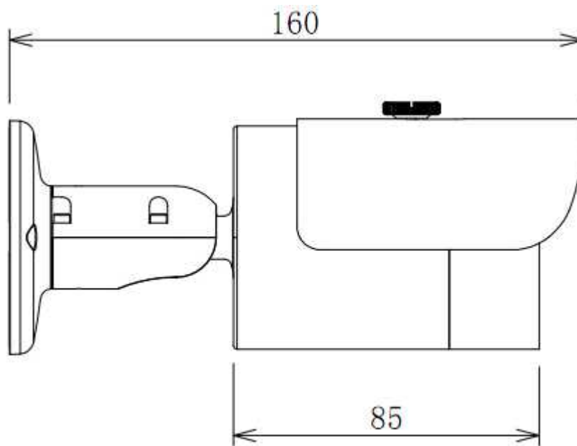
Figure 2-2 Dimension illustration 1
