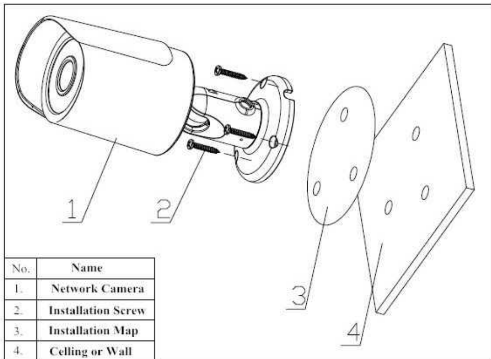
Figure 3-1 Device installation 1
