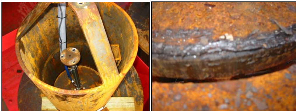
Fig. 4.5 Dummy turbine condition (31.03.03) and severe erosion of dummy turbine gate (11.08.03)
