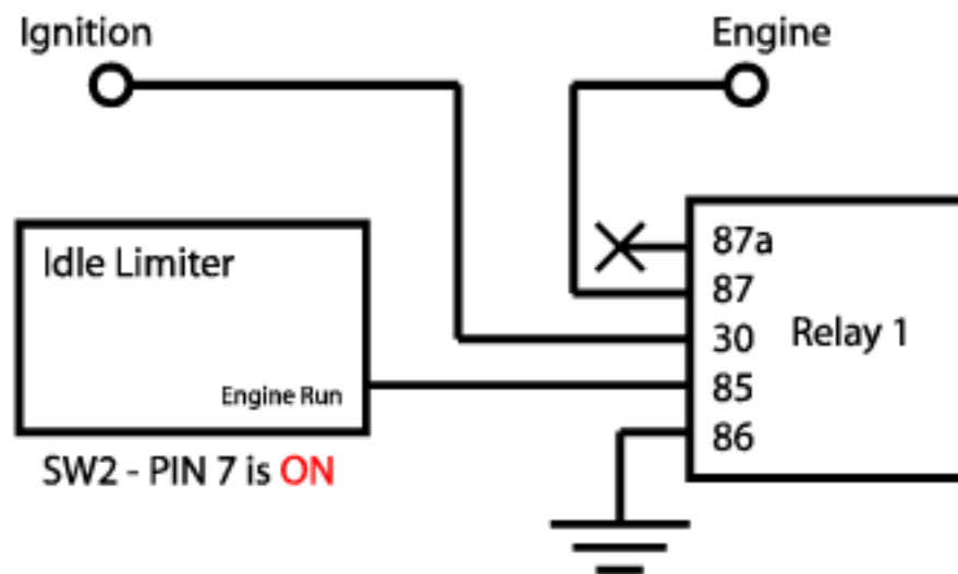
Relay Configuration 2
