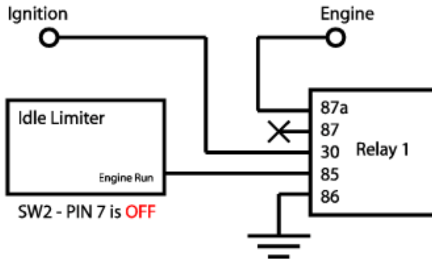
Relay Configuration 1
