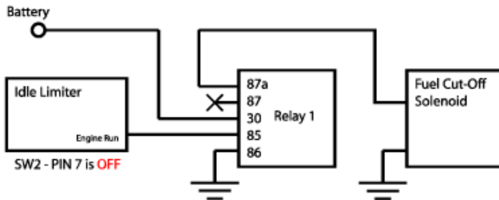
Relay Configuration 4
