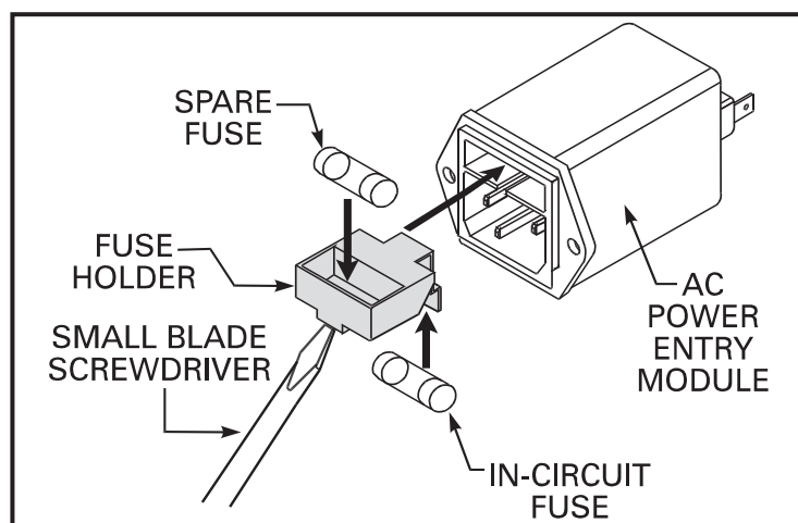
Figure 22. Installing a Fuse
