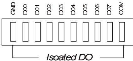
Figure 2.5: Digital Output Connector Pin Assigns
