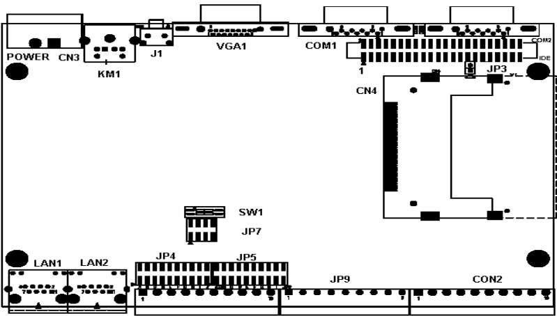
Figure A.1: Connector & Jumper Locations (Top)
