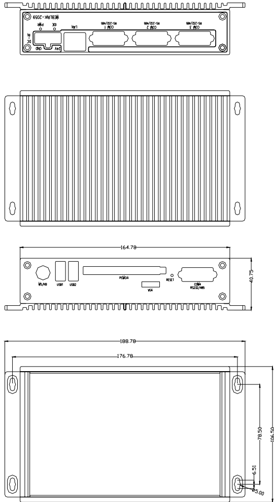
Figure 1.1: Chassis Dimensions
