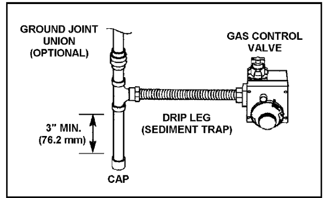
FIGURE 19. GAS PIPING WITH FLEXIBLE CONNECTOR.
