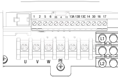
Single Phase (2/PE) 240 VAC models with Filter and/or integrated line disconnect
