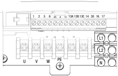
Single Phase (2/PE) 120/240 VAC models (ESVxxxN01SMC) with integrated line disconnect
