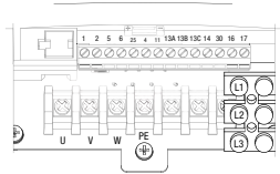
Three Phase (3/PE) models with Filter and/or integrated line disconnect
