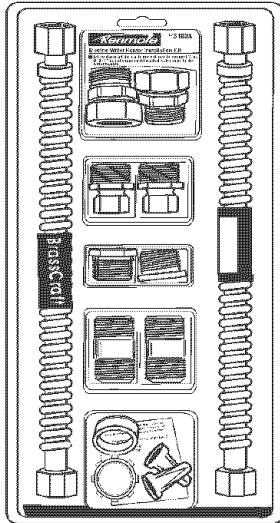
WATER HEATER INSTALLATION KIT WITH FLEXIBLE CONNECTORS FOR 3/4" OR 1/2" THREADED OR COPPER PLUMBING.
