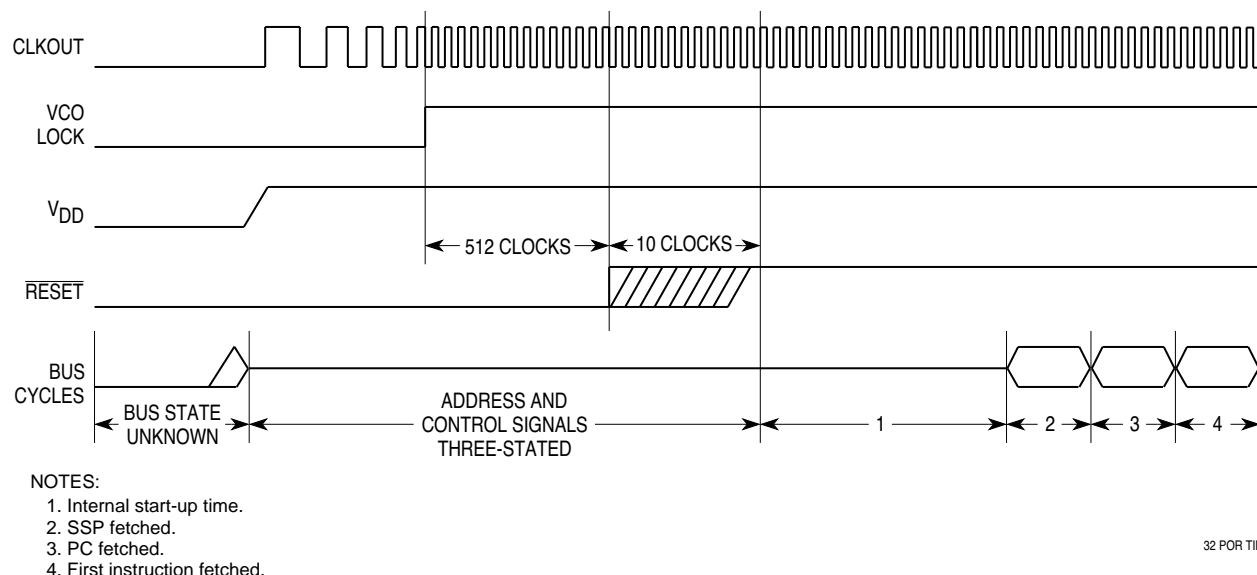
Figure 4-16 Power-On Reset
