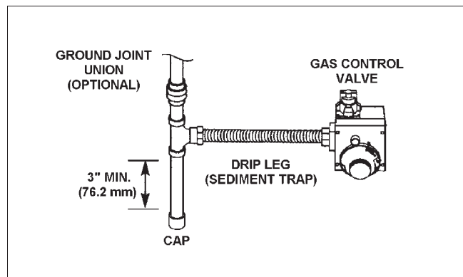
FIGURE 20. GAS PIPING WITH FLEXIBLE CONNECTOR.
