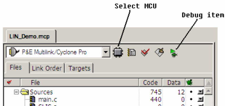
Figure.1 CodeWarrior interface
