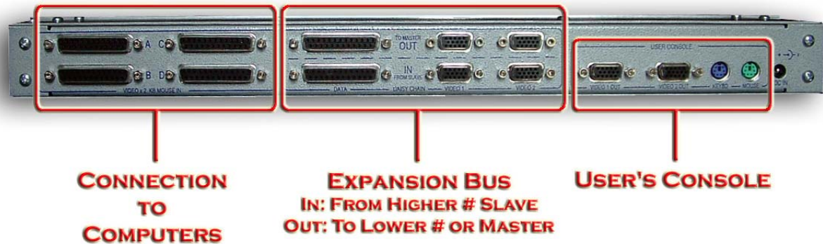
FIGURE 1 MC4-H2 Connector Functions on Rear Panel
