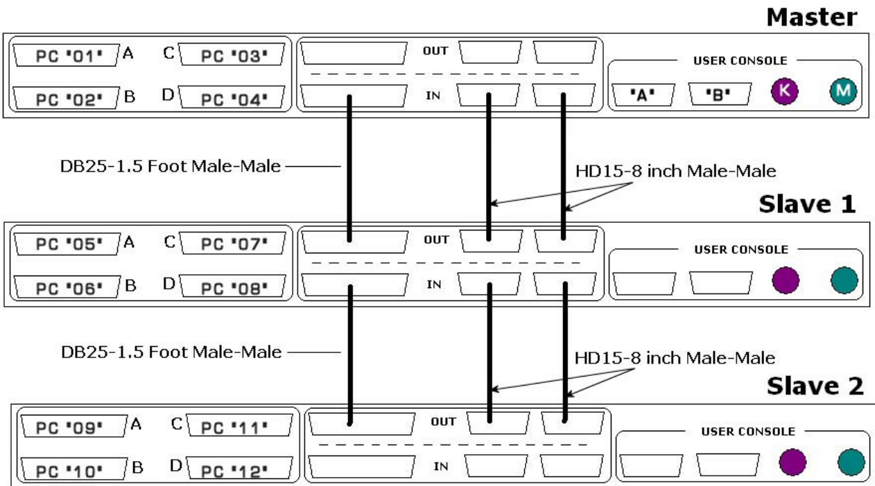
FIGURE 3 Stacking of MC4-H2 or MC4-H2-SW Units
