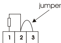
2 wires probe
