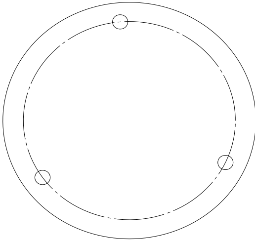
Fig 2.2.4 Fix card
