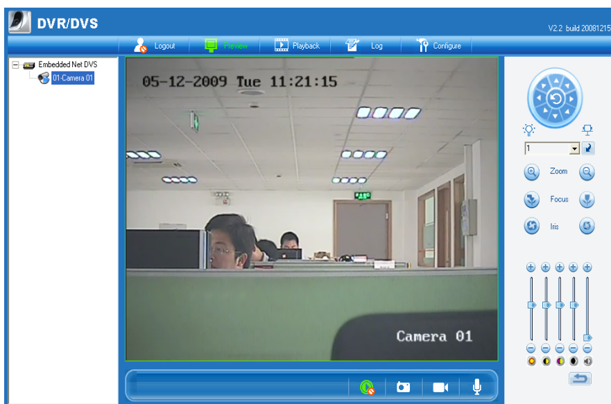
Fig 3.5 Preview Interface
