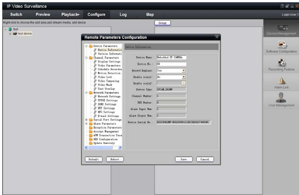
Fig.3.2.11 Remote Configuration
