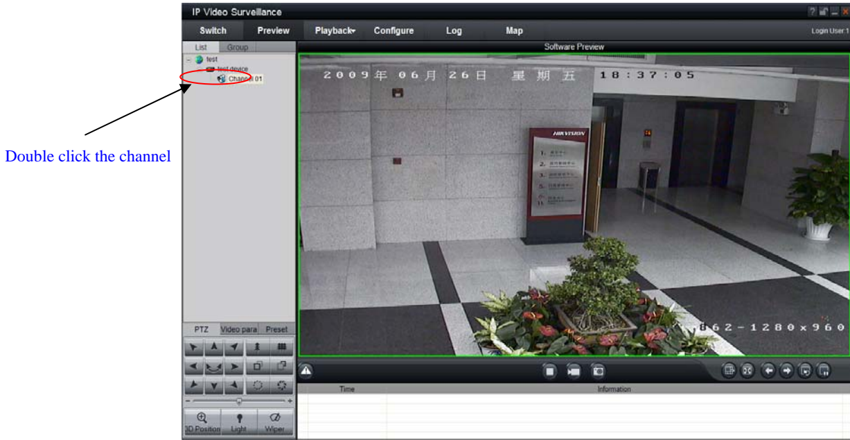
Fig.3.2.10 Preview Menu
