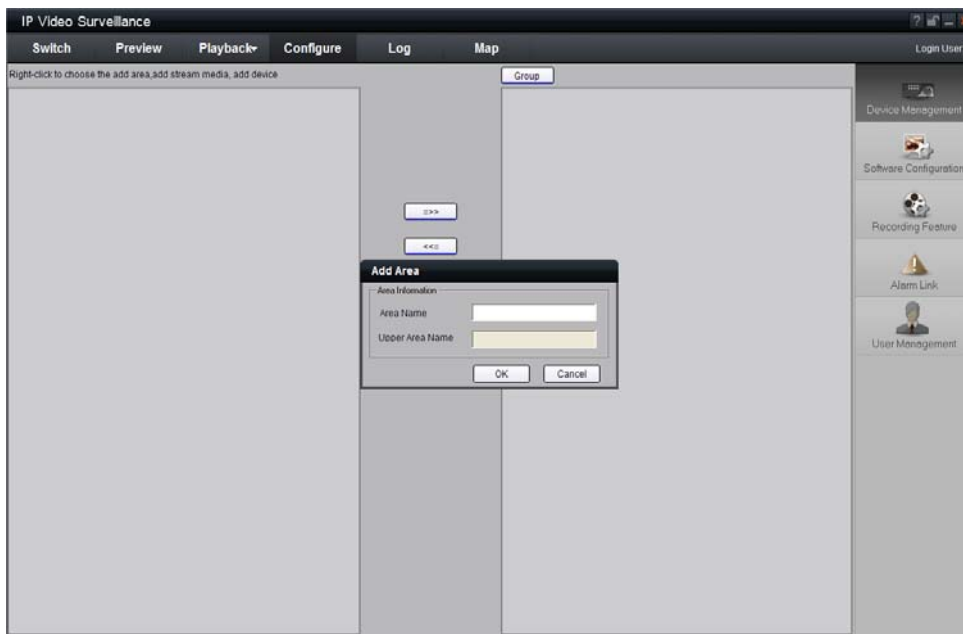
Fig. 3.2.5 Area Properties
