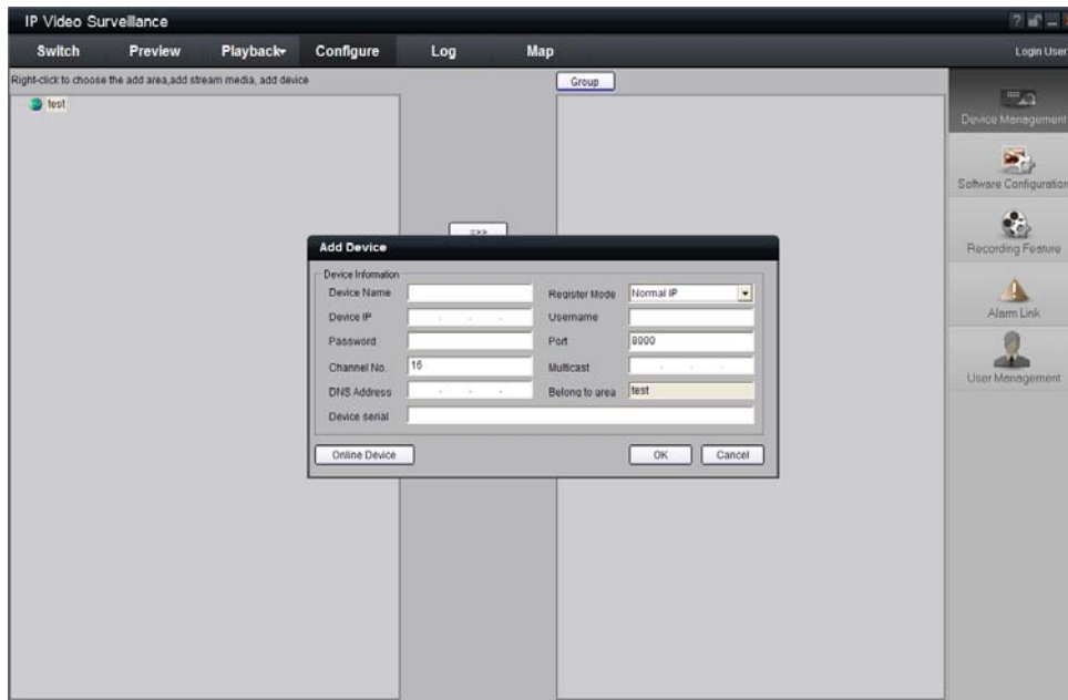
Fig. 3.2.8 Add Device
