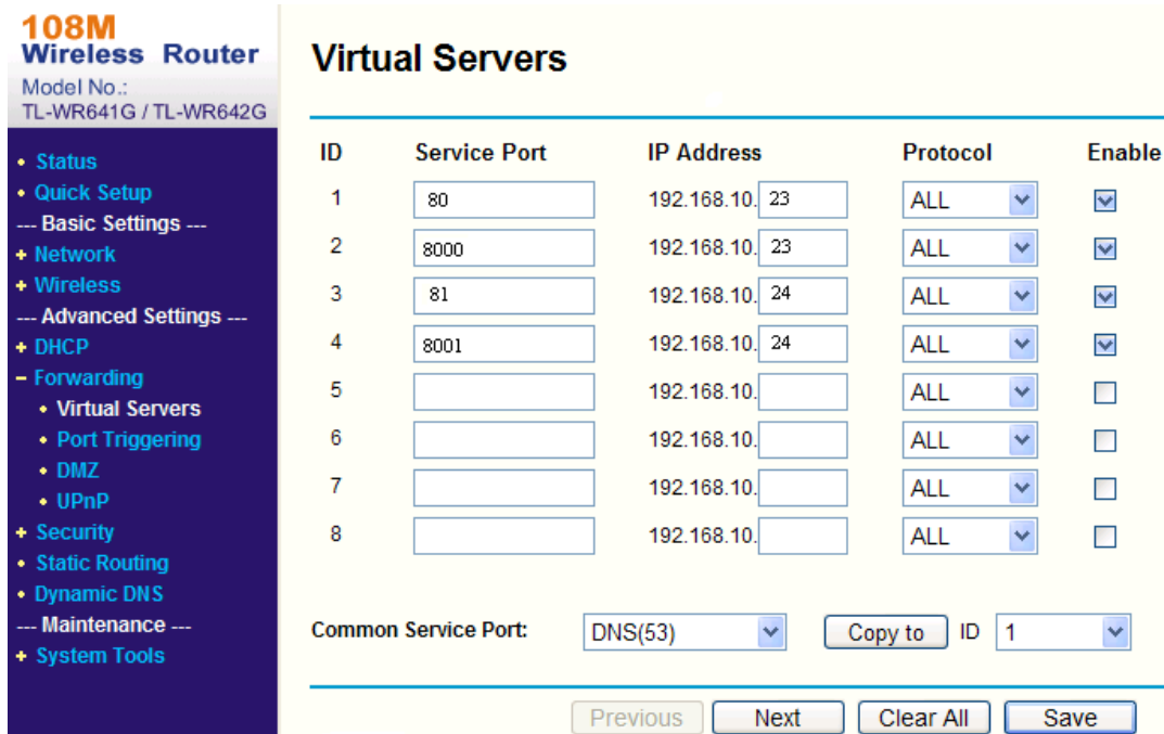
Fig.4.3 Port mapping
