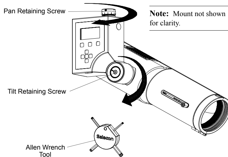
Figure 1: PL1 Luminaire Pan & Tilt Adjustment
