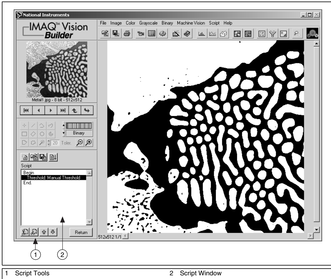
Figure 2-4. Thresholded Image
