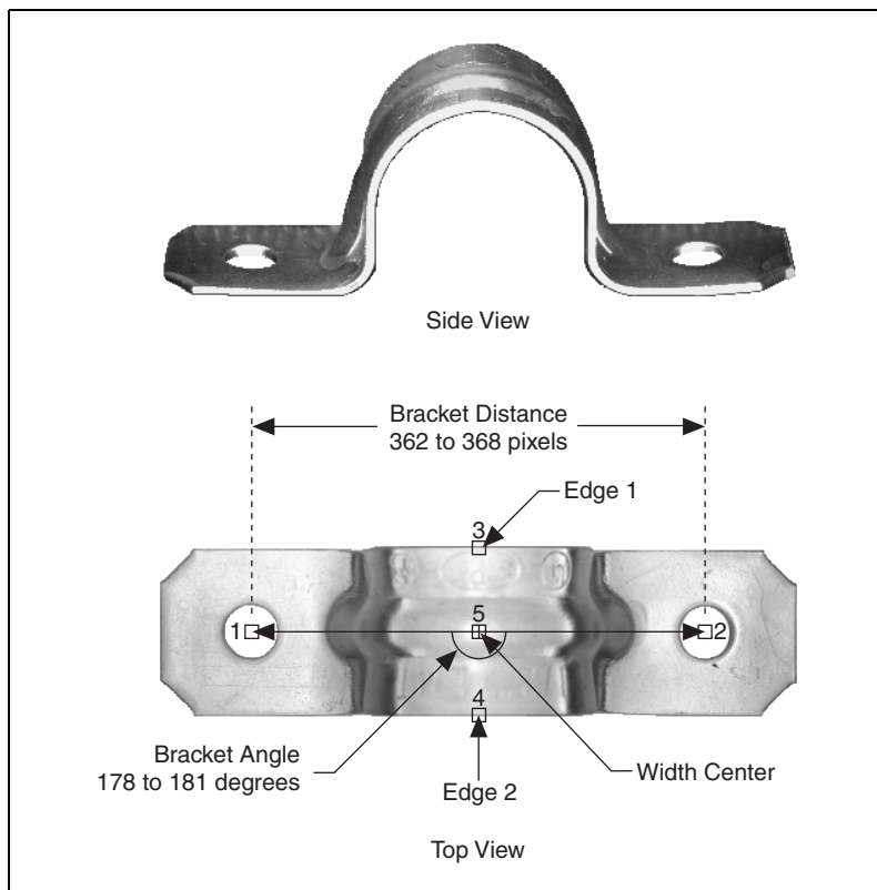
Figure 4-1. Bracket Specifications
