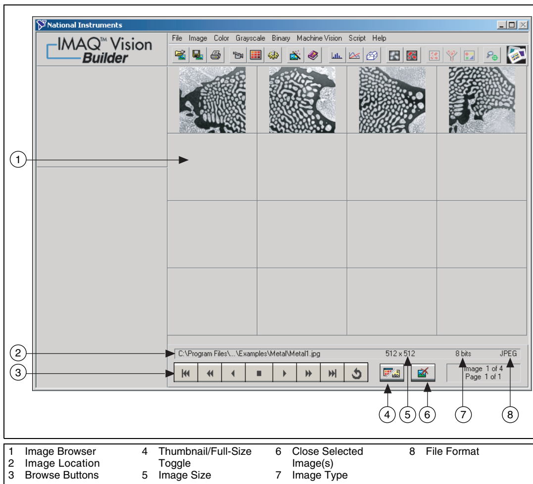
Figure 2-1. Image Browser
