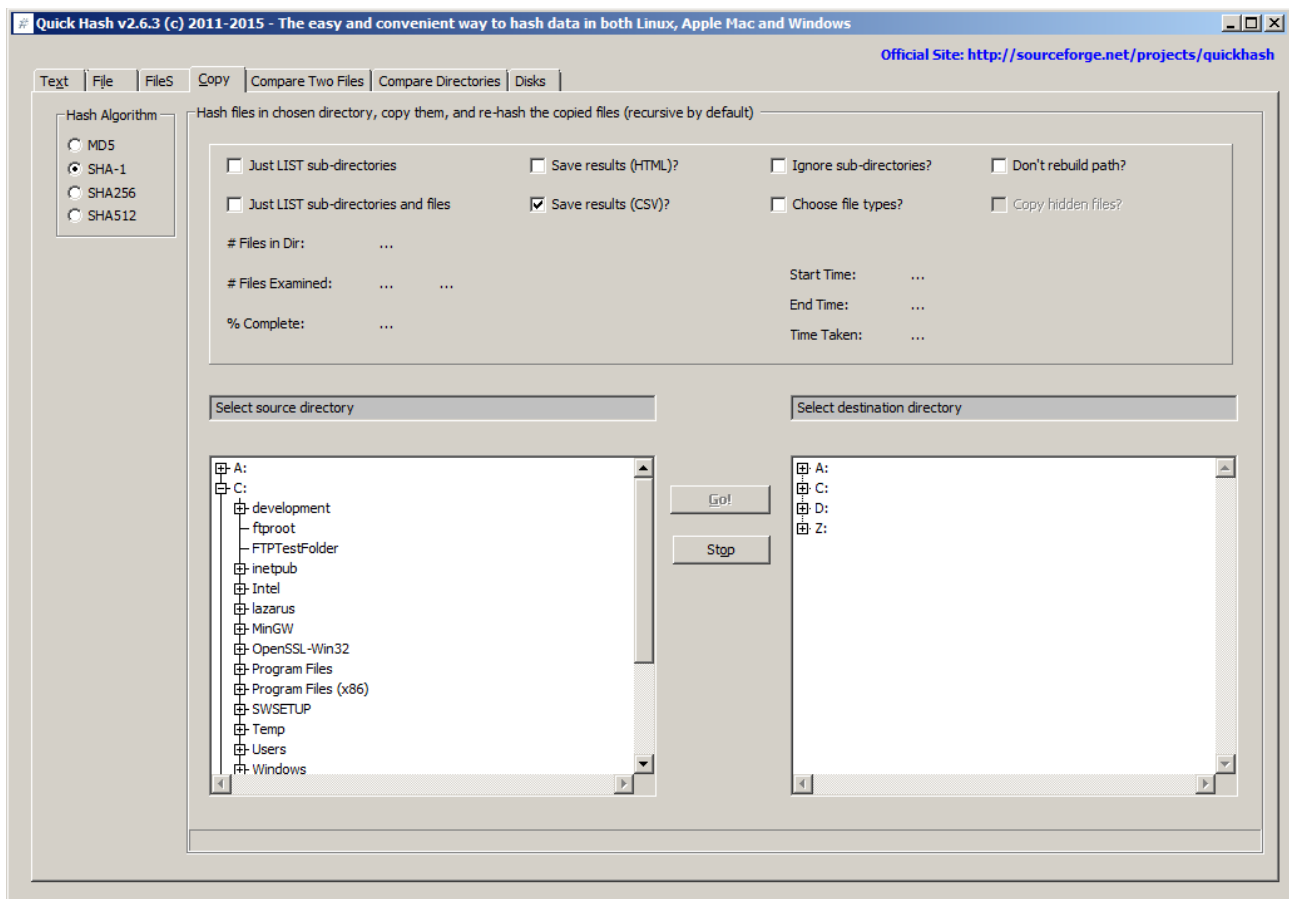
Illustration 8: The default 'Copy' tab showing tree views (new feature as of v2.6.3)
