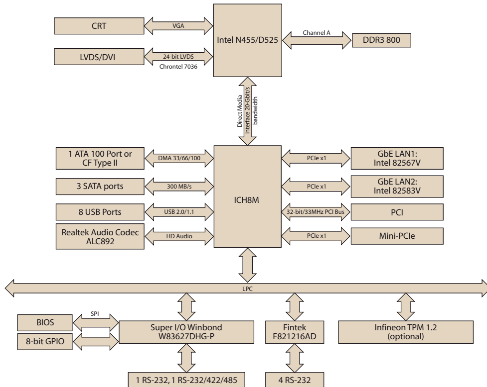
Figure 1.3 AIMB-213 Board Diagram
