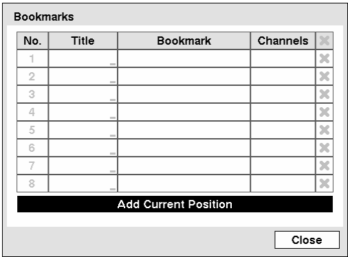
Figure 120 — Bookmarks screen.
