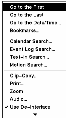
Figure 118 — Search menu.
