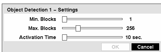
Figure 89 — Settings screen.
