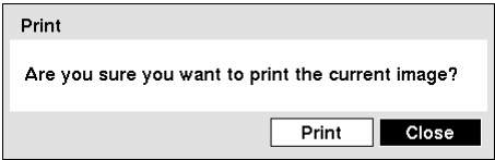
Figure 129 — Print screen.
