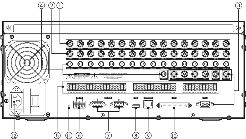
Figure 2 — Rear panel.
