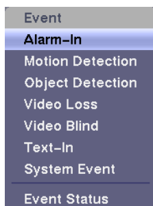
Figure 73 — Event menu.
