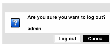
Figure 42 — Logout screen.
