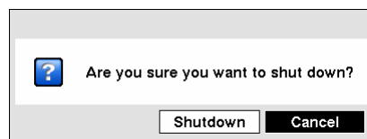
Figure 41 — Shutdown screen.
