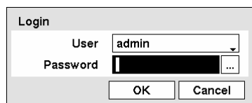
Figure 23 — Login screen.
