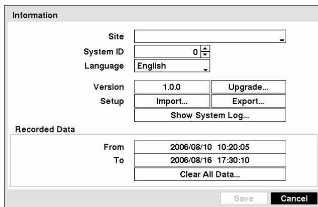
Figure 26 — Information screen.
