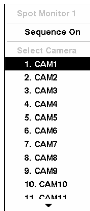
Figure 113 — Sequence menu.
