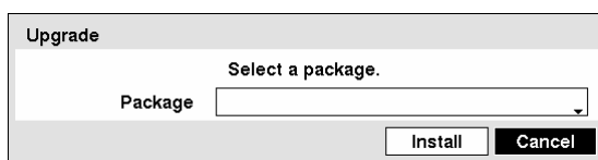
Figure 27 — Upgrade screen.
