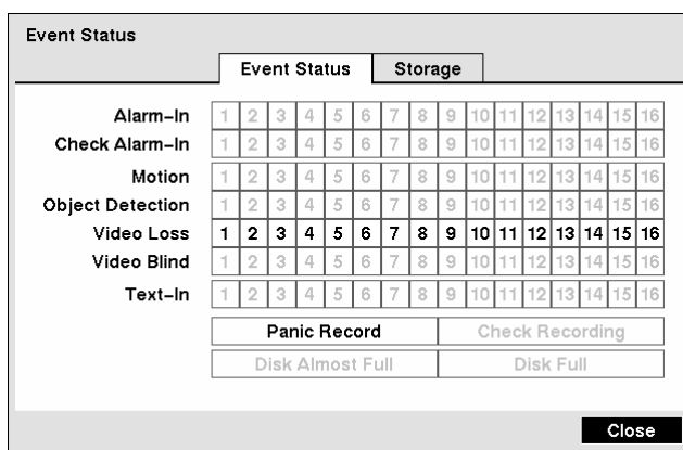
Figure 107 — Event Status screen.
