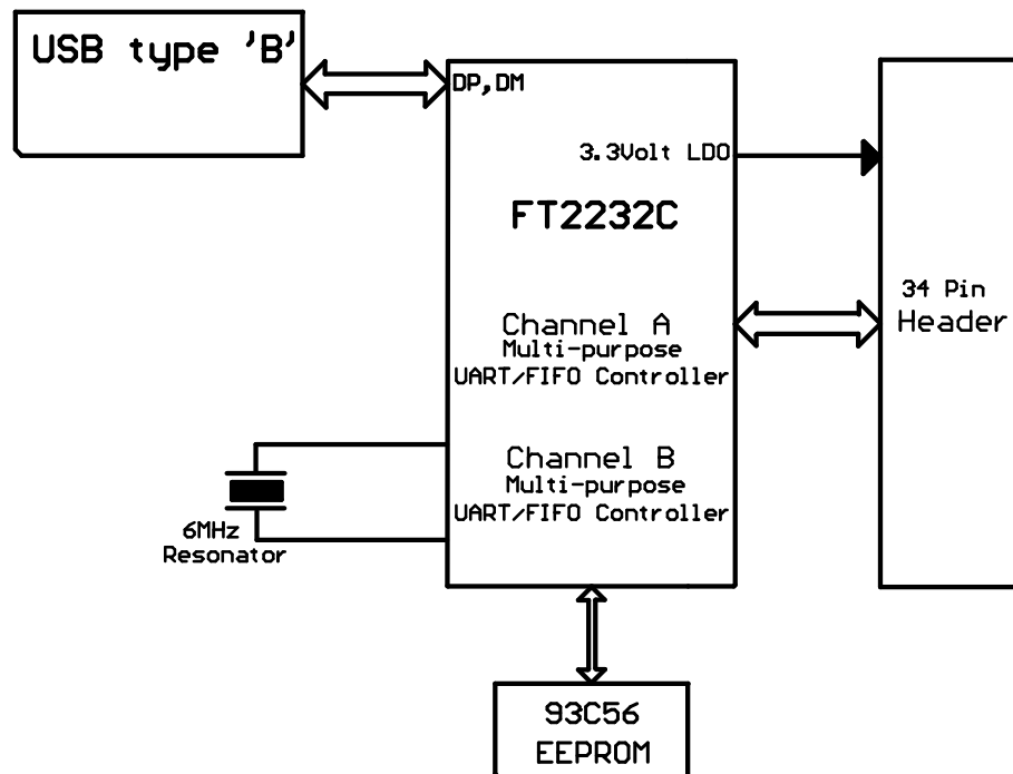
Figure 1. MMusb2232 block diagram.
