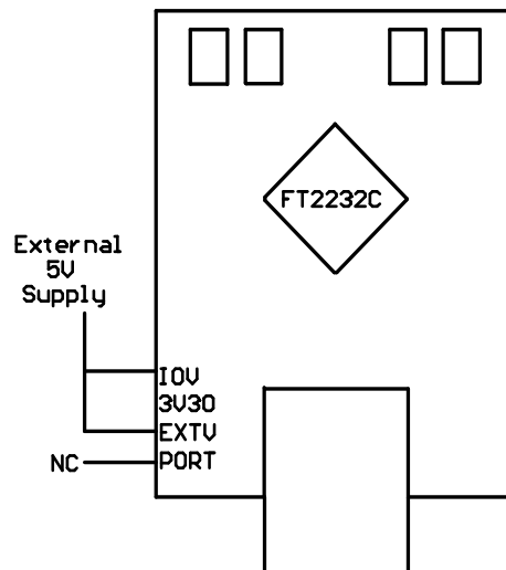
Figure 3b.Self Powered Configuration
