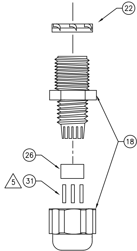
DETAIL B
