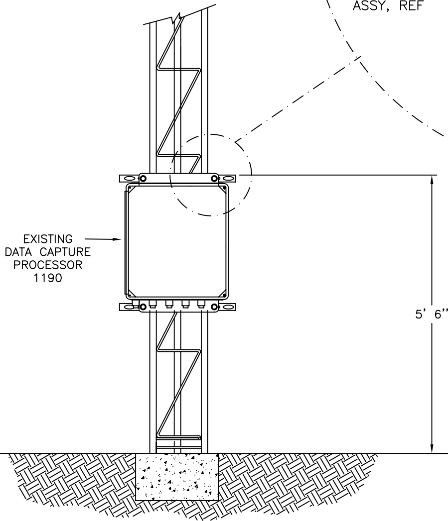
MOUNTING KIT, ENCLOSURE TO TOWER M488119-01
