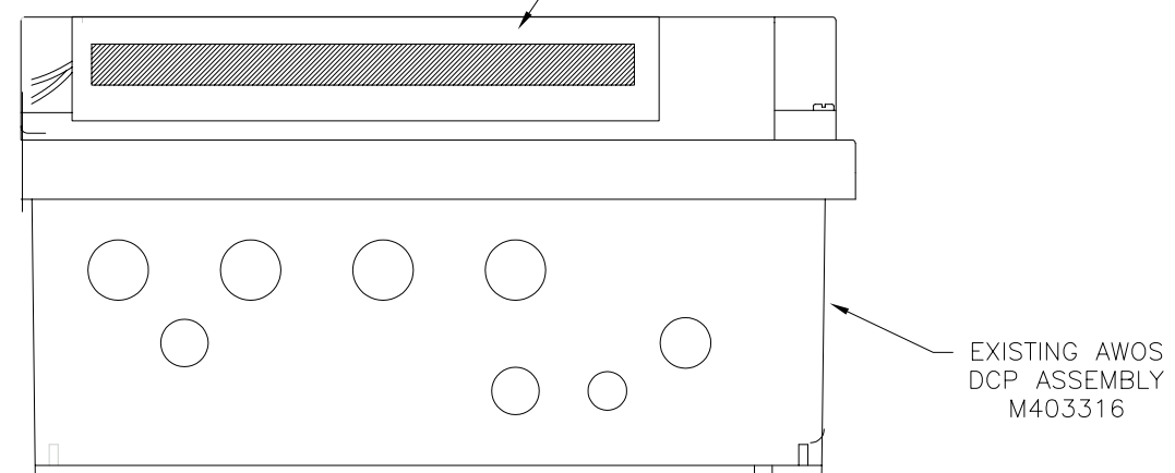
ENCLOSURE BOTTOM VIEW ENCLOSURE LID SHOWN AS A SECTION FOR CLARITY
