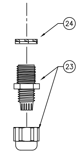
DETAIL C
