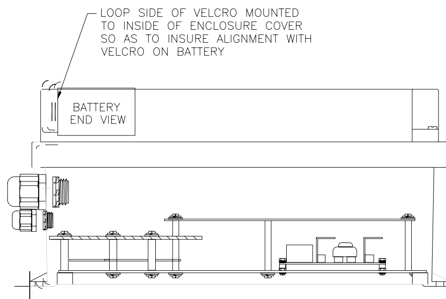
ENCLOSURE SIDE VIEW SECTION
