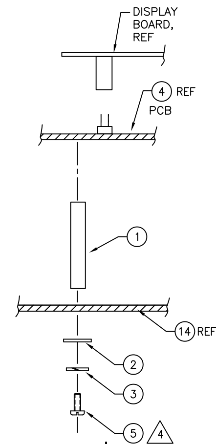
DETAIL L
