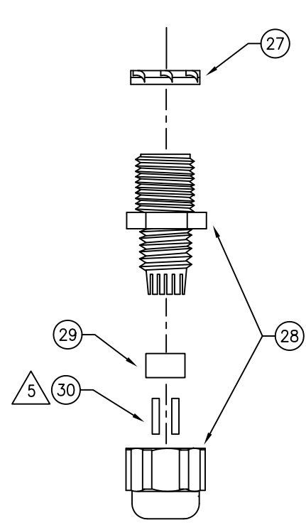
DETAIL A
