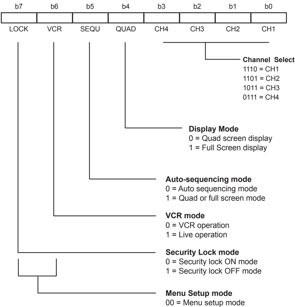
BYTE 1: Status code for normal operation modes
