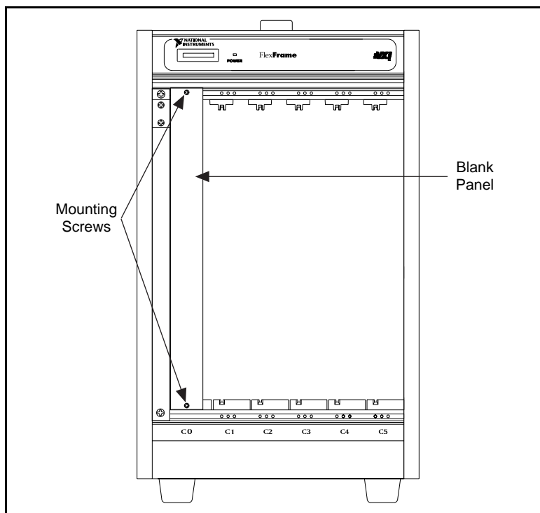
Figure 2-3. Filler Panels
