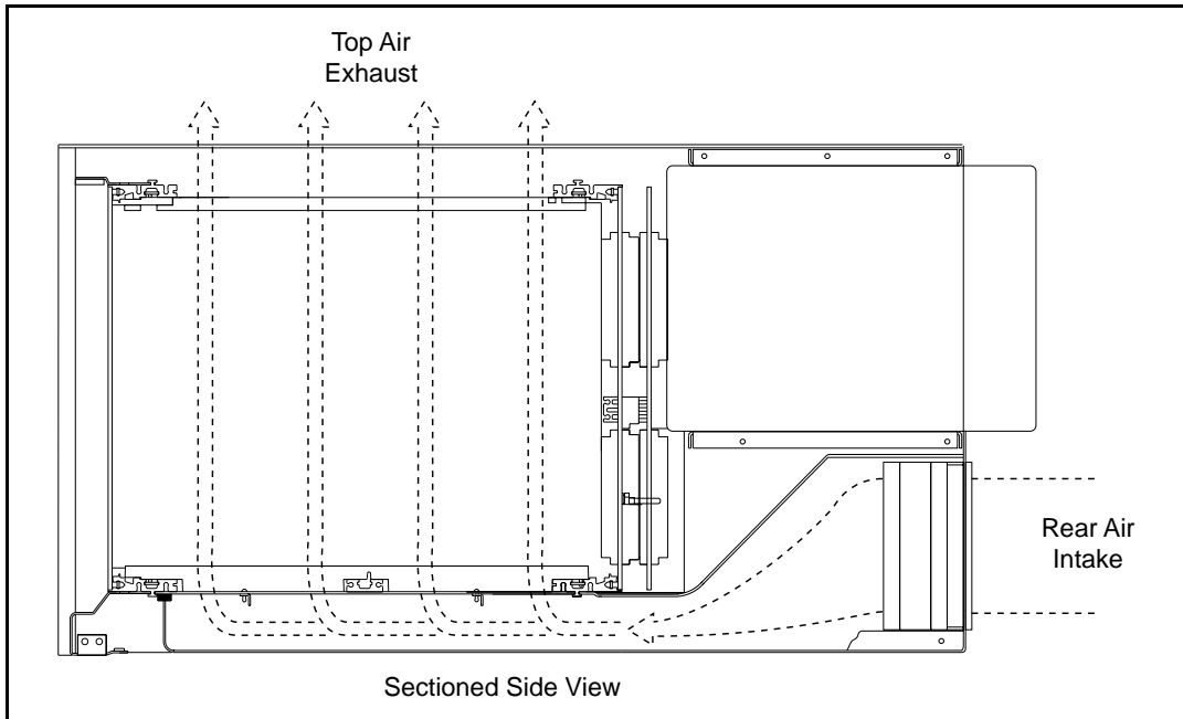
Figure 1-6. VXI-1200 Bench-Top Configuration Positive-Pressure Cooling System
