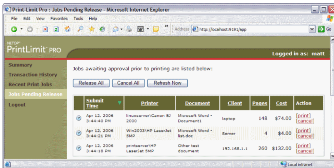
Figure 10.4. End-user web-based interface listing held jobs
