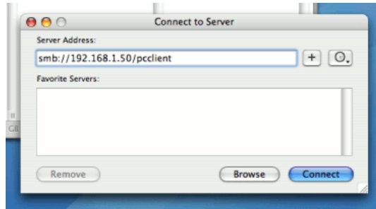
Figure 22.27. The PCClient share's connection string
