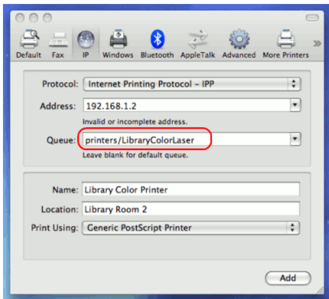
Figure 22.3. Setting up a workstation printer on Leopard
