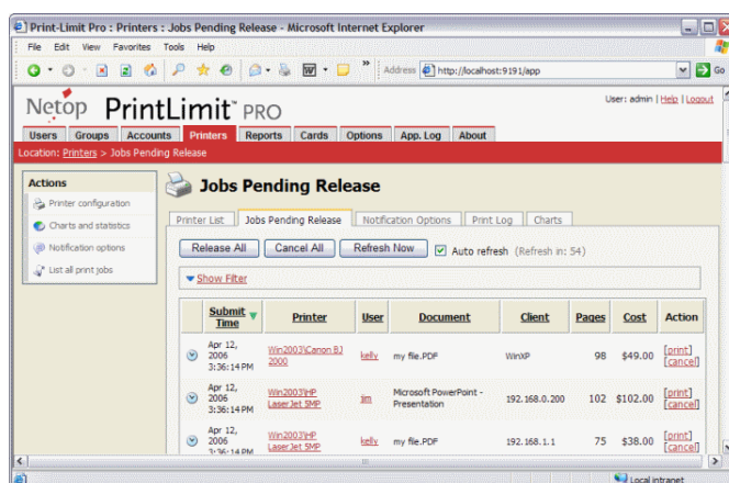
Figure 10.3. Web-based release station within the admin pages
