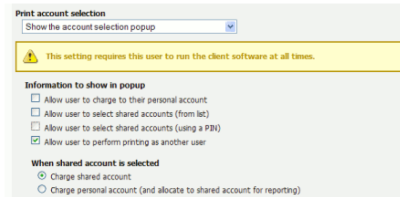
Figure 23.3. Enable perform printing as other user
