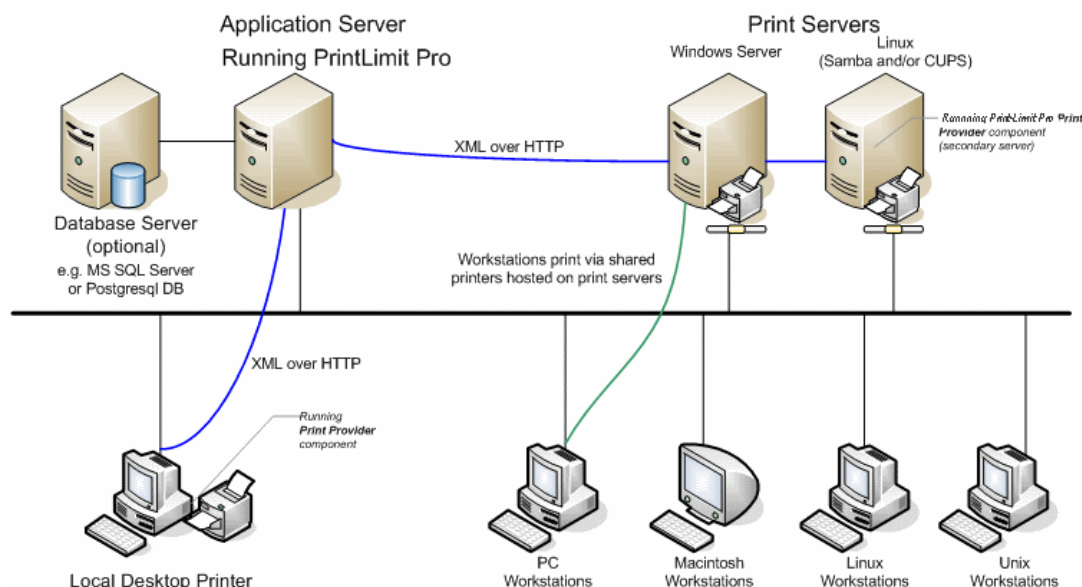
Figure 14.2. Print-Limit Pro Architecture - an advanced configuration
