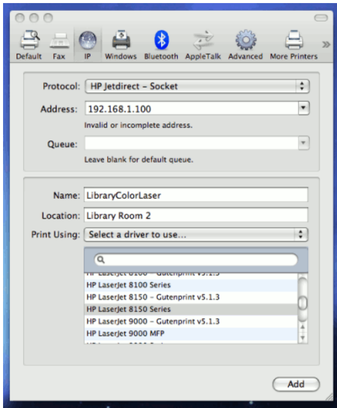
Figure 22.1. Setting up a printer (direct) on Leopard server using Jetdirect
