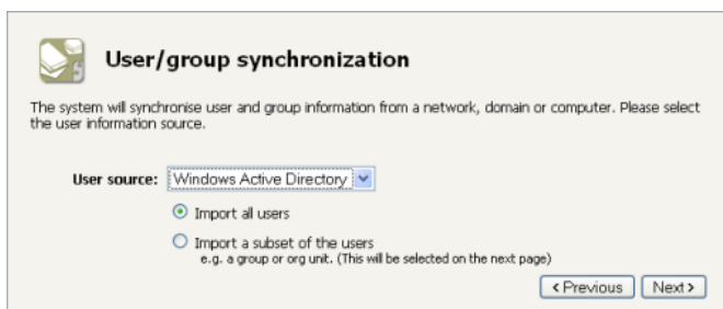
Figure 2.5. User sync configuration wizard page
