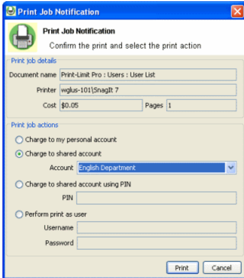
Figure 8.13. Selecting a shared account from the popup
