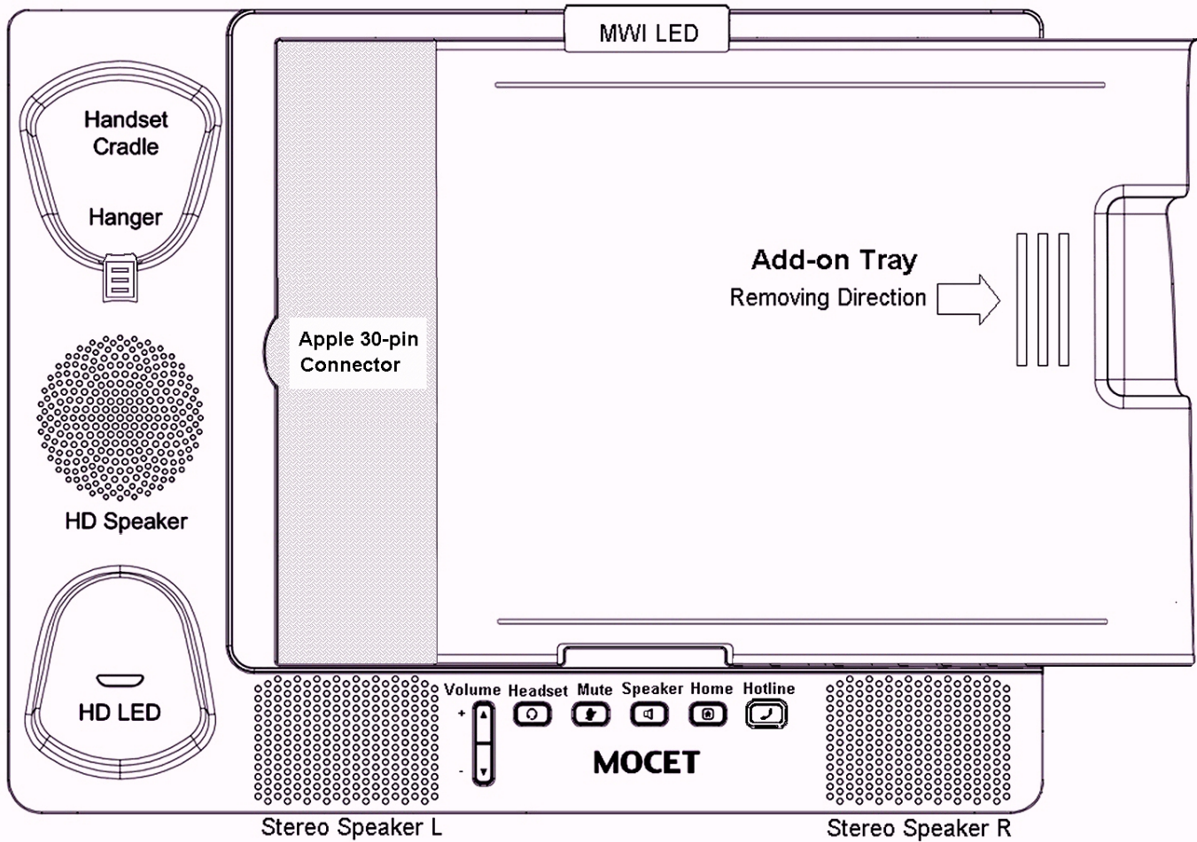
Figure 3. The Communicator Front Appearance and Add-on Tray
