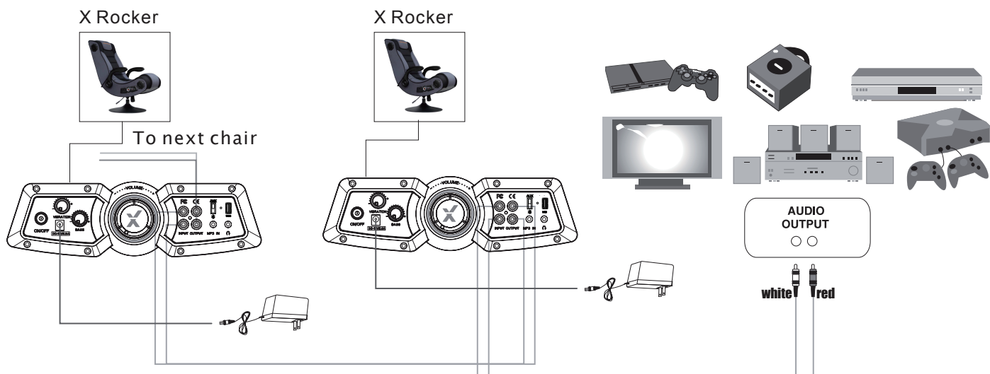
DIAGRAM 4 MULTI-USER CONNECTION
