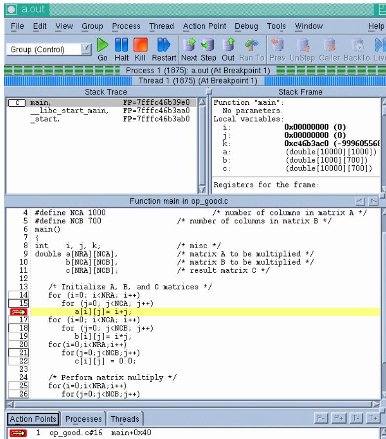
Figure 3-2 TotalView Session
