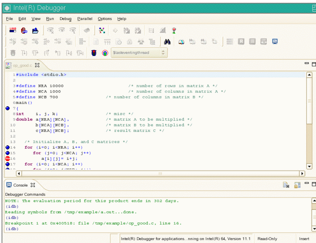
Figure 3-1 Intel® Debugger GUI
